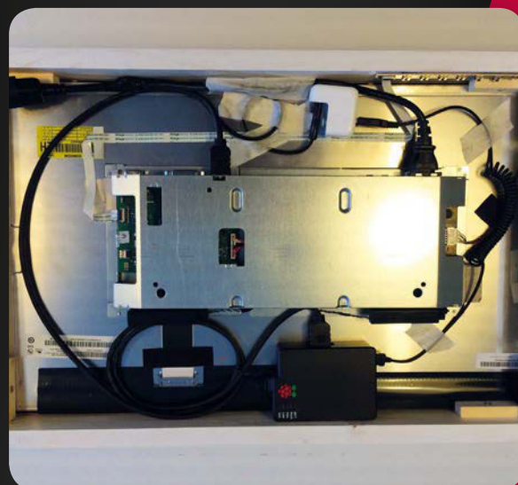
The hardware inside the mirror is quite simple (and relatively cheap)
