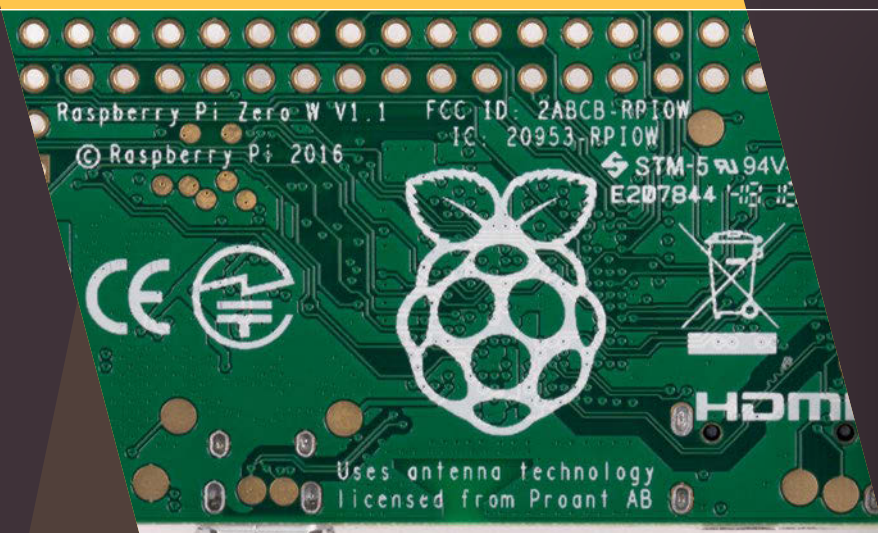
The white text is added to the PCB using a silk-screen technique. These markings are used to provide information and branding for the board.
