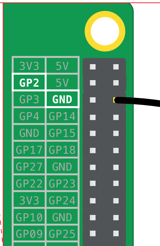
Fig 2 If you have an older Raspberry Pi model you'll only have 26 pins, but they have the same layout
