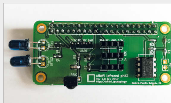
Below The Infrared pHAT is perfectly designed to sit on top of a Pi Zero
