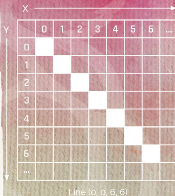
Figure 1 The coordinates system in Processing moves right and down, rather than right and up as in traditional Cartesian coordinate systems
