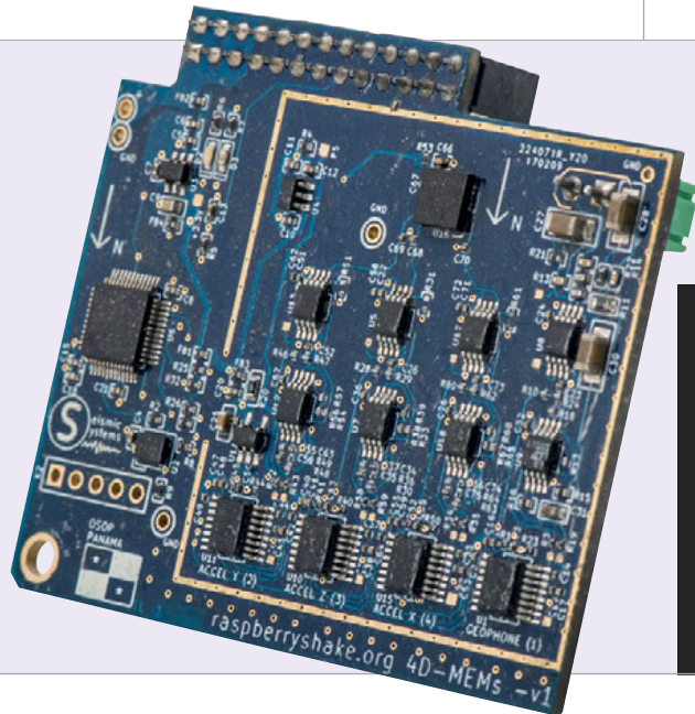
The Raspberry Shake board converts the analogue signal from the geophone into a digital signal, and works with the Raspberry Pi to process the data for you to view and analyse
