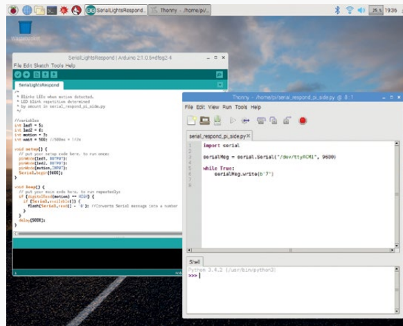
Left The Arduino sketch (on the left) includes a serial read function that gets data from the Python code (on the right)
