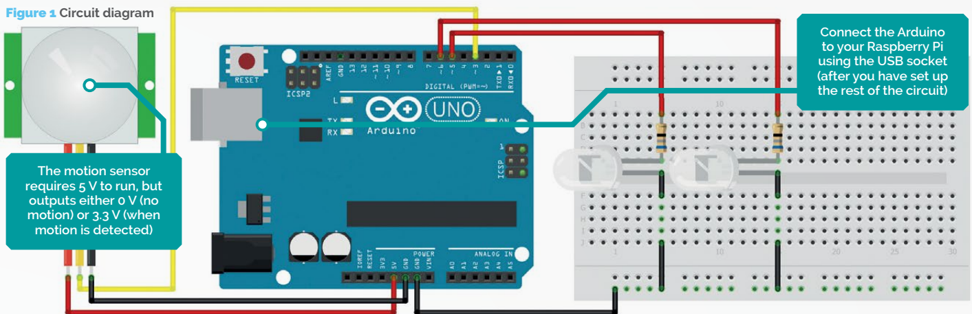
Figure 1 Circuit diagram
