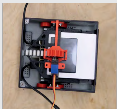
Right The cartridge looks like a Polaroid picture, and is ejected using a rack-and-pinion mechanism
