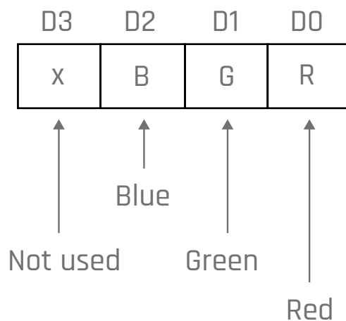
Figure 2 LED control
