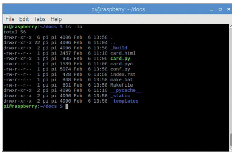
Figure 3 The file structure of Sphinx once it’s all installed
