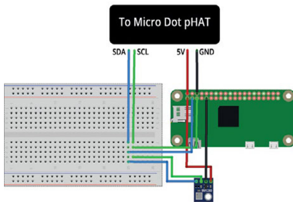
Above The BME280 is connected to 3V, GND, SDA, and SCL pins on the Pi. The Micro Dot pHAT is connected to 5V, GND, SDA, and SCL as well
