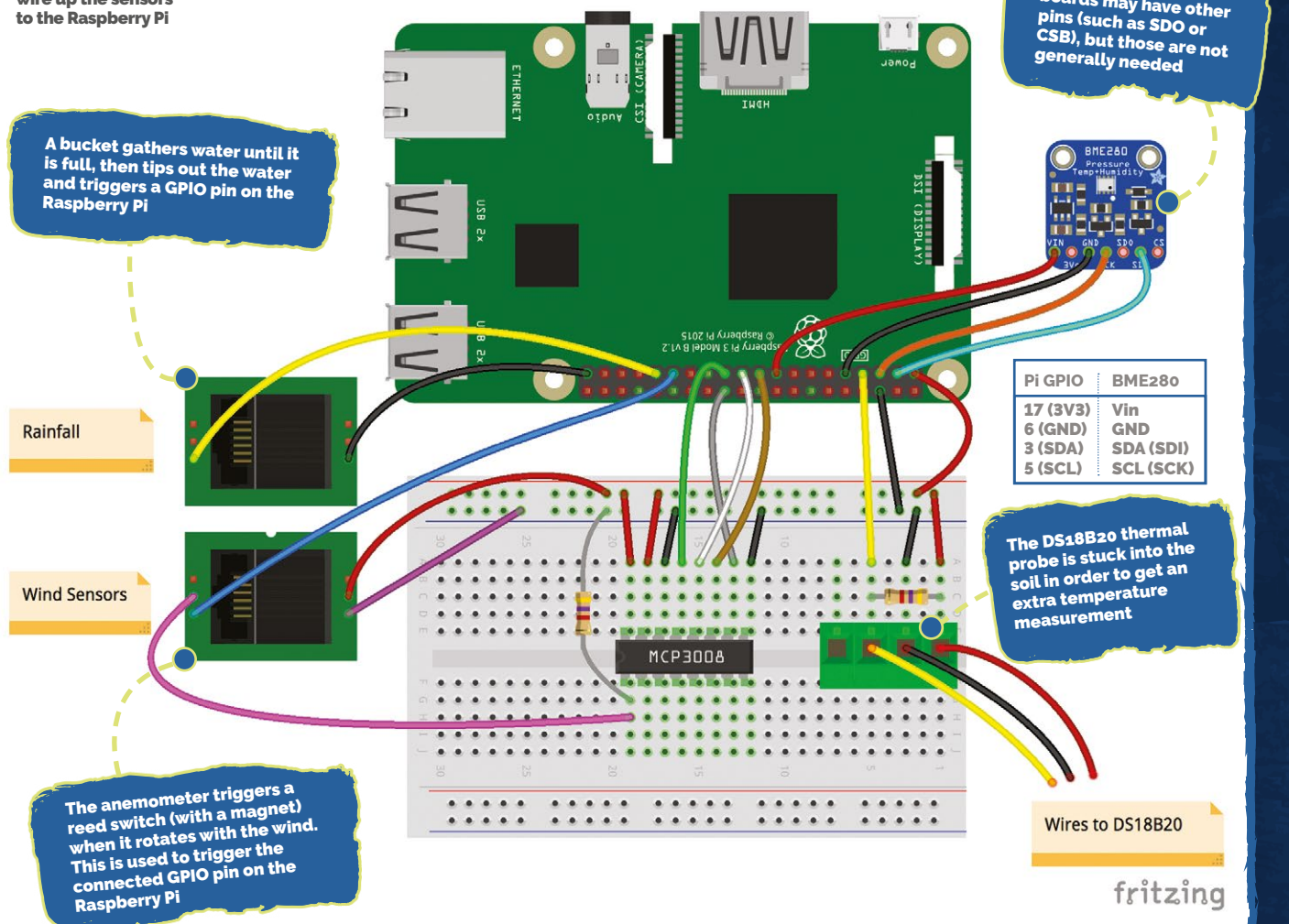
Figure 1 How to wire up the sensors to the Raspberry Pi
