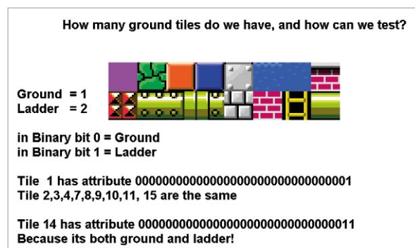
Figure 4 Encoding tile attributes into bit fields
