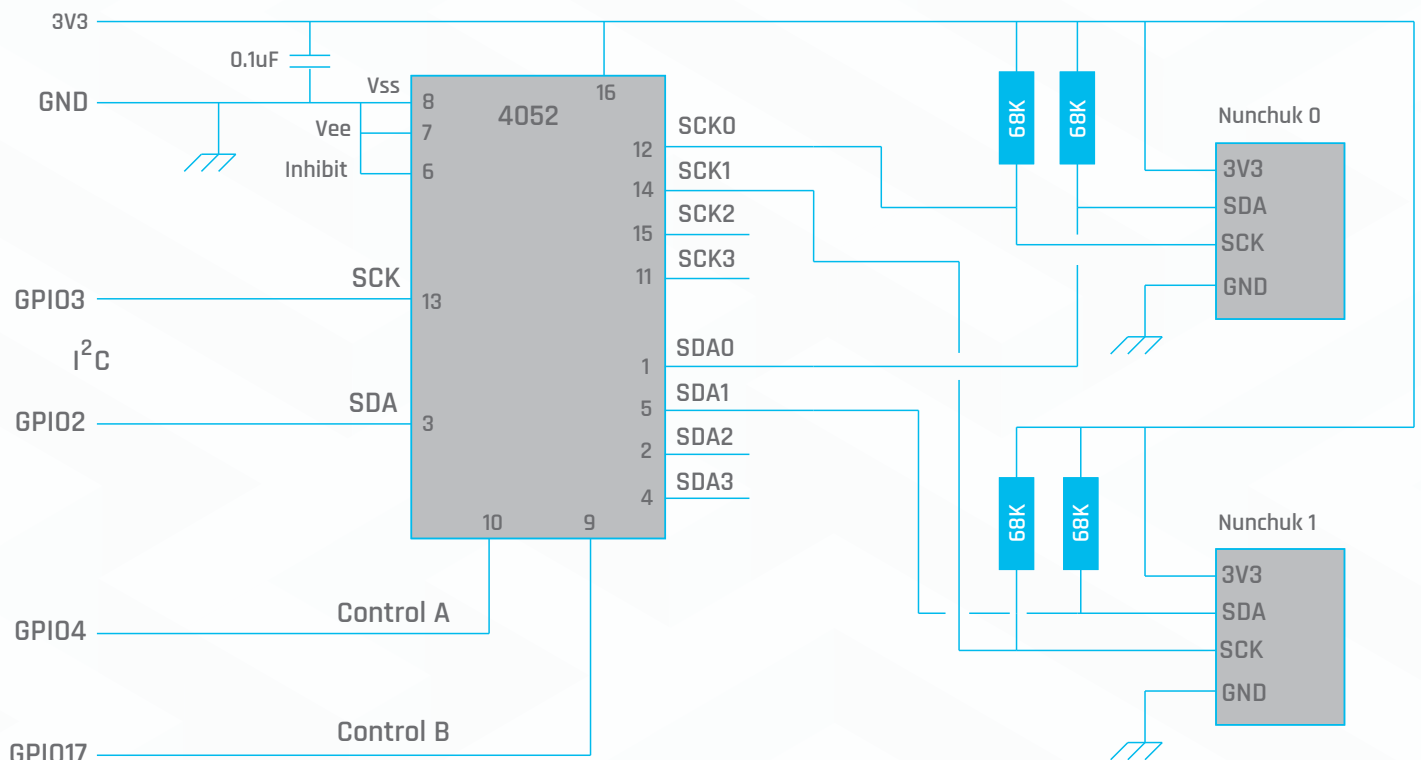
Figure 1 Schematic of the I²C multiplex board
