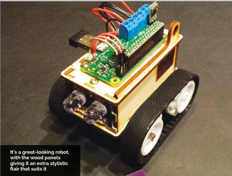
The board with the LEDs is custom-made, to cut down on wiring in the project
