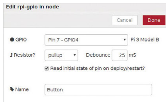
Figure 7 Adding a button input is easy
