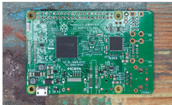
Above The world's thinnest Raspberry Pi 3. Image credit: Pimoroni
