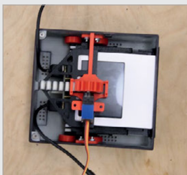
Right The cartridge looks like a Polaroid picture, and is ejected using a rack-and-pinion mechanism
