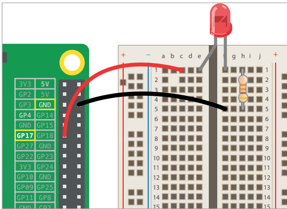
Figure 1 Wire up an LED to GPIO 17 – make sure you use the 330 \Omega resistor as shown
