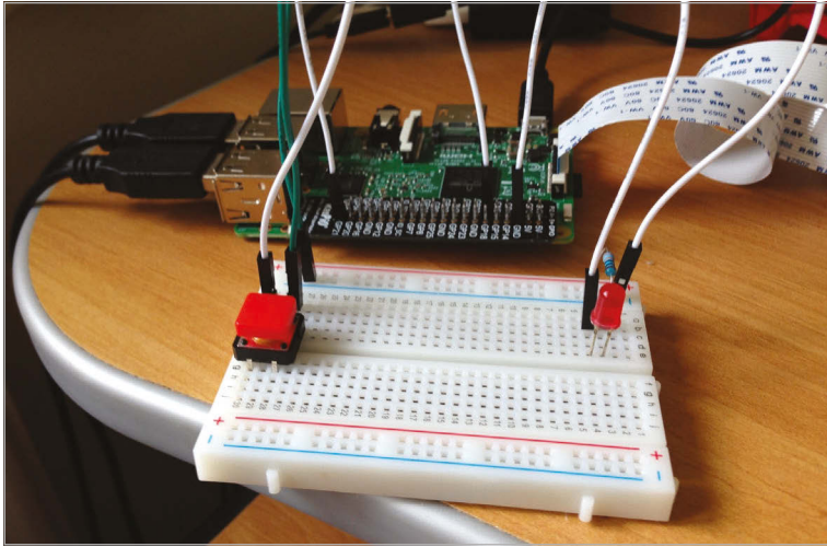
Above: This project is simple to wire up using a solderless breadboard and some jumper wires
