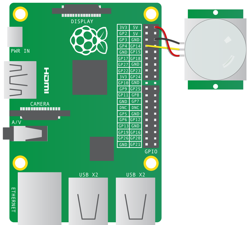
Above How to wire a PIR sensor up to a Raspberry Pi
