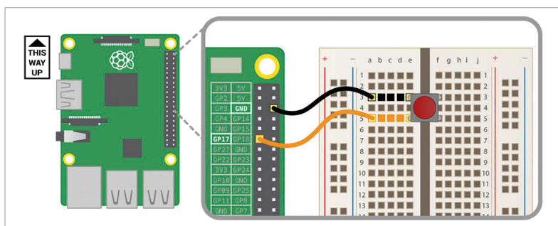
Fig 1 Connect your button to pin 17 and a ground pin. If you don't have a button, make one by tapping your two bits of wire together
