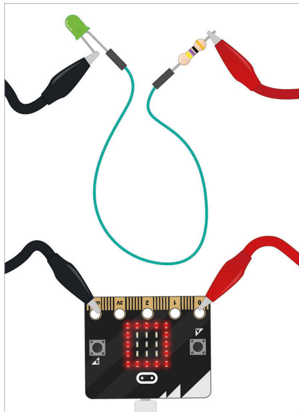
Fig 1 The GPIO pins in the micro:bit allow students to control physical components such as LEDs
