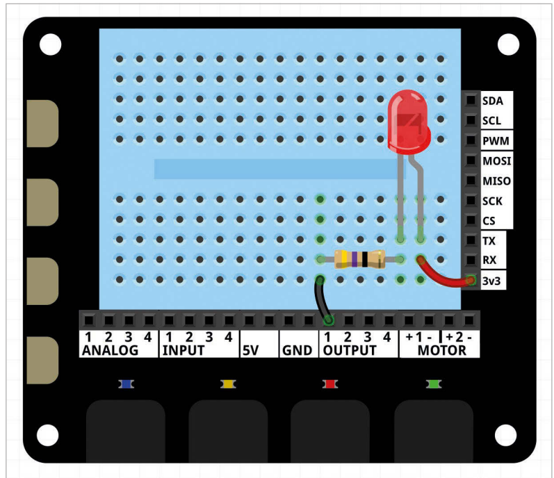
Fig 1 Using the built-in breadboard to wire up an LED to a digital output, using a 47Ω resistor
