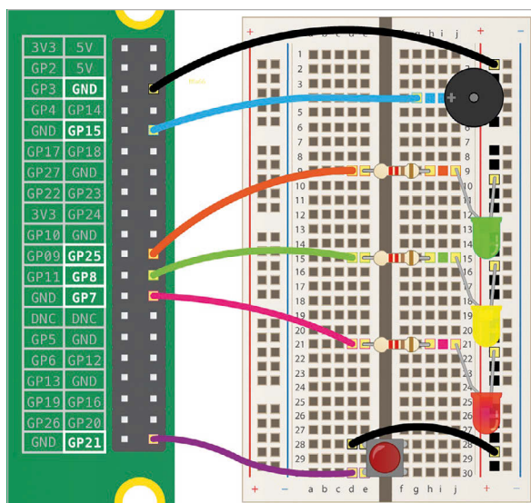
A circuit containing three LEDs, a button, and a buzzer, to simulate traffic lights
