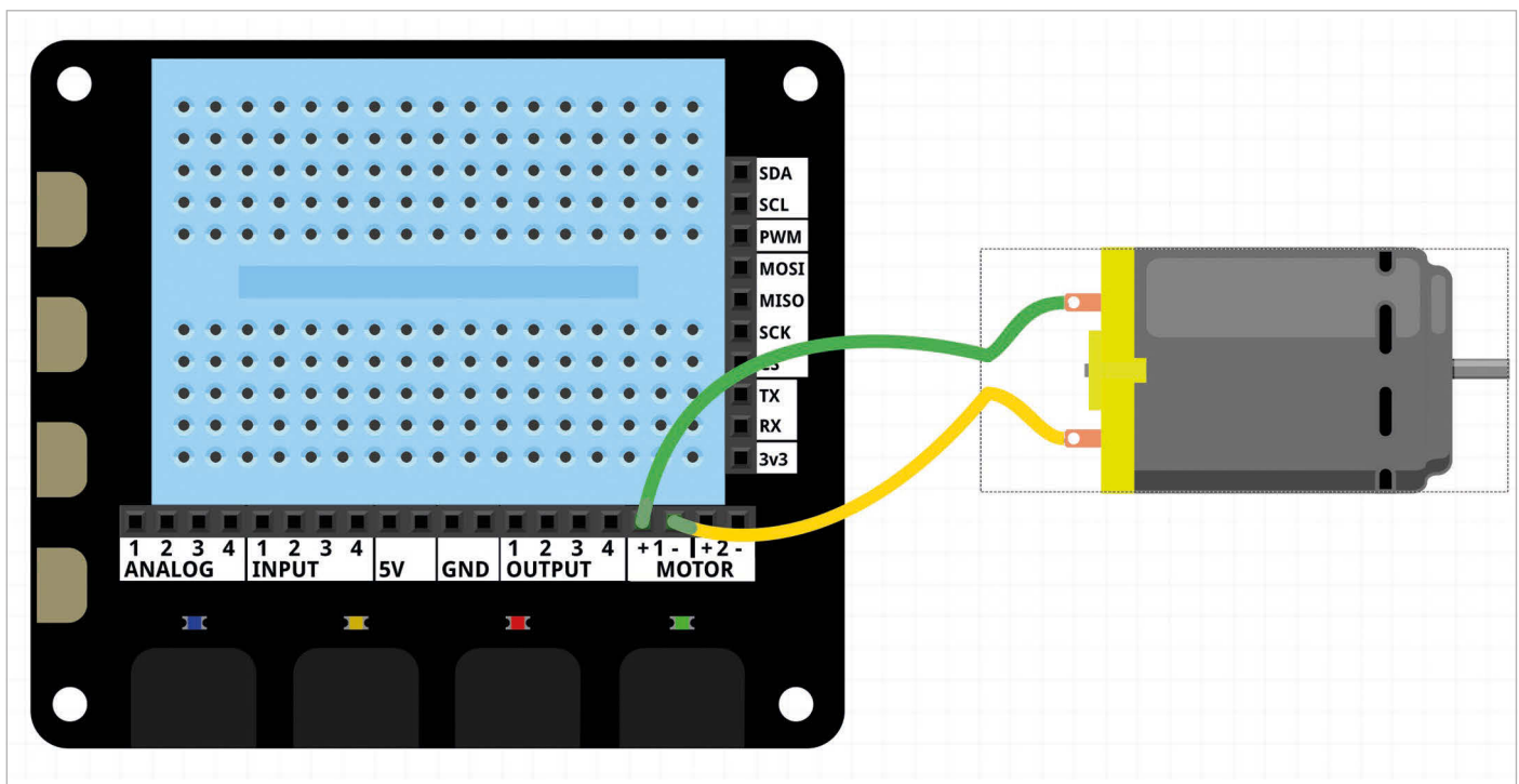
Fig 3 Wiring a motor directly to the 5V motor output pins on the Explorer HAT Pro
