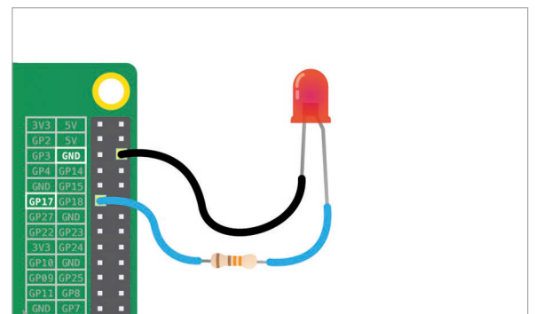
A single LED connected to the Raspberry Pi using jumper leads and a resistor
