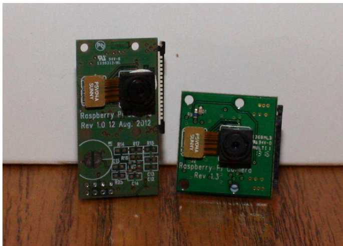
Prototype camera board (left) and final camera board (right)
