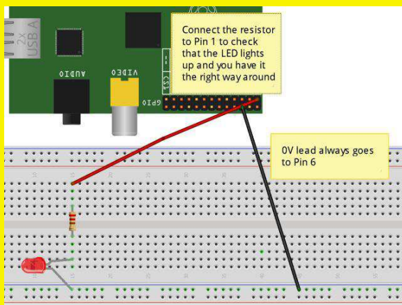
Figure 1 - LED Test
