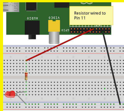
Figure 2 - GPIO Test
