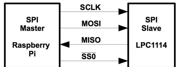
Figure 1 MSPI Connections
