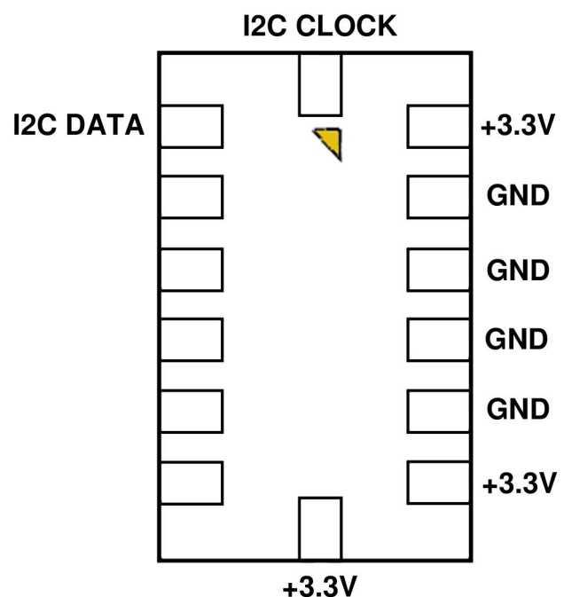
MMA7455 (BOTTOM)
