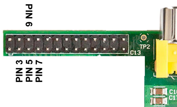
Raspberry Pi Physical Pins
