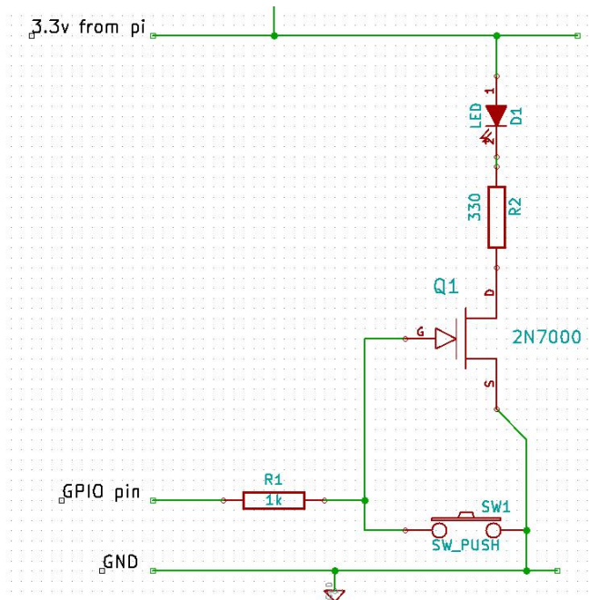
Figure 1: FET Buffer
