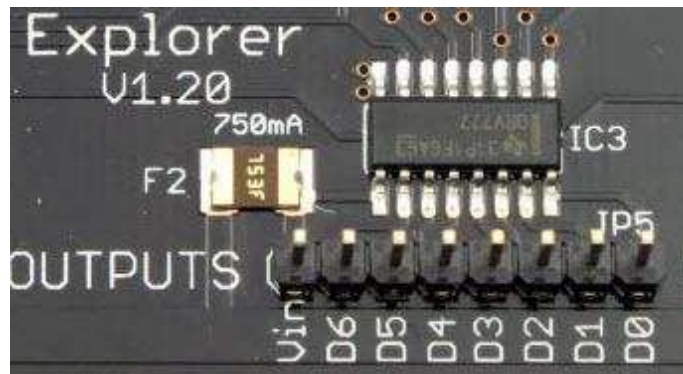
Figure 2.0 - Digital outputs on the Explorer
