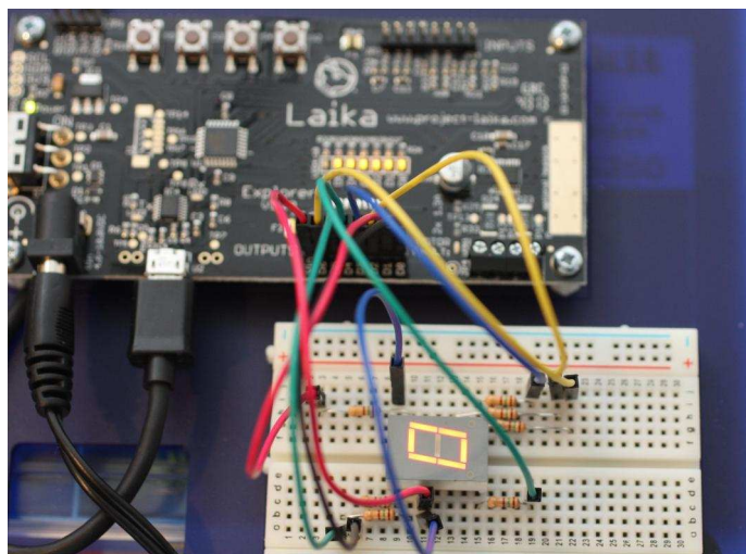
Figure 7.0 – 7-segment control
