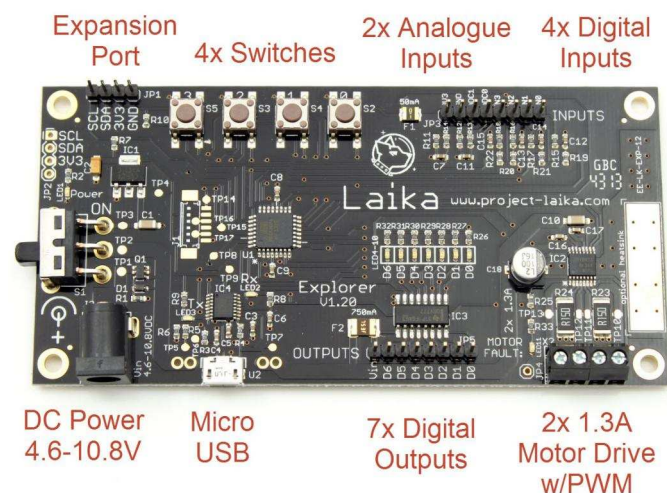
Figure 1.0 - The Laika Explorer V1.20
