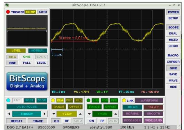
Figure 5: Determining the frequency of a signal
