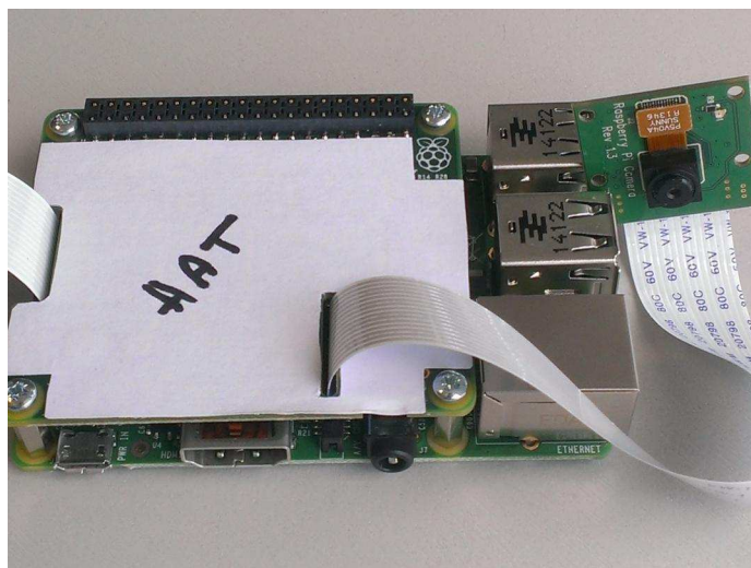
Model B+ Raspberry Pi with mechanical sample of HAT board
