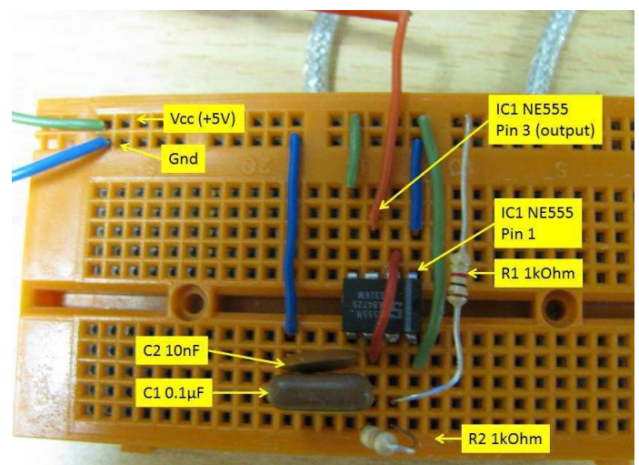
Fig. 6: Implementation on a breadboard
