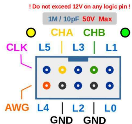
Fig. 2: Pin layout of the BitScope Micro (photo courtesy by BitScope Designs)
