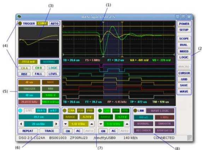
Fig. 1: BitScope DSO software main screen elements (photo courtesy by BitScope Designs)
