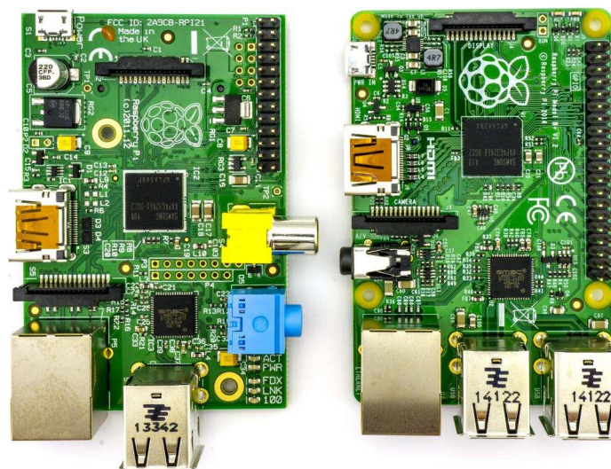
Comparison between Model B and Model B+ boards
