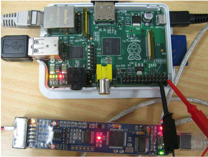
Fig. 3: Measuring +5V on the GPIO pins 2 and 6 of the Raspberry Pi
