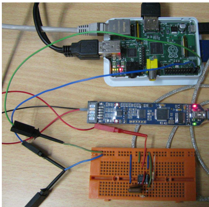
Fig. 7: Connecting the clock generator to the Raspberry Pi and BitScope Micro
