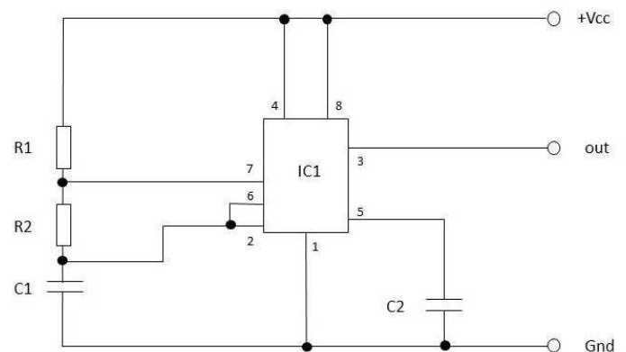
Fig. 5: Circuit diagram of the clock generator
