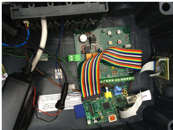
Raspberry Pi and Matboard controlling a water pump
