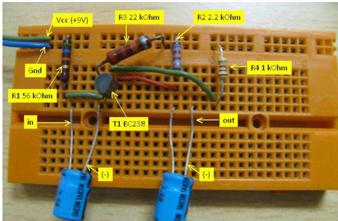
Fig. 6: Single transistor pre-amplifier built on a breadboard
