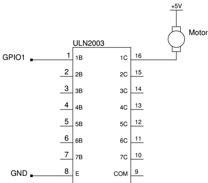
Figure 2 - ULN2003 and small DC motor
