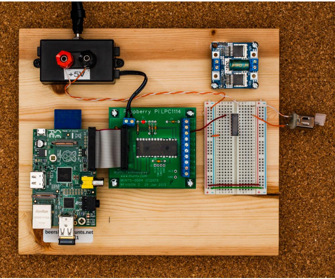
Figure 3 - Small DC motor test stand
