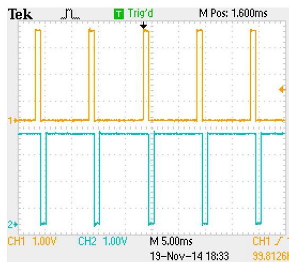
Figure 1 - Pulse width modulation signals
