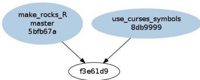
Figure 2: The repo history after our first merge.
