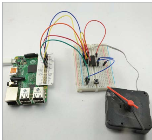
Above Tick tock... everything is wired up
