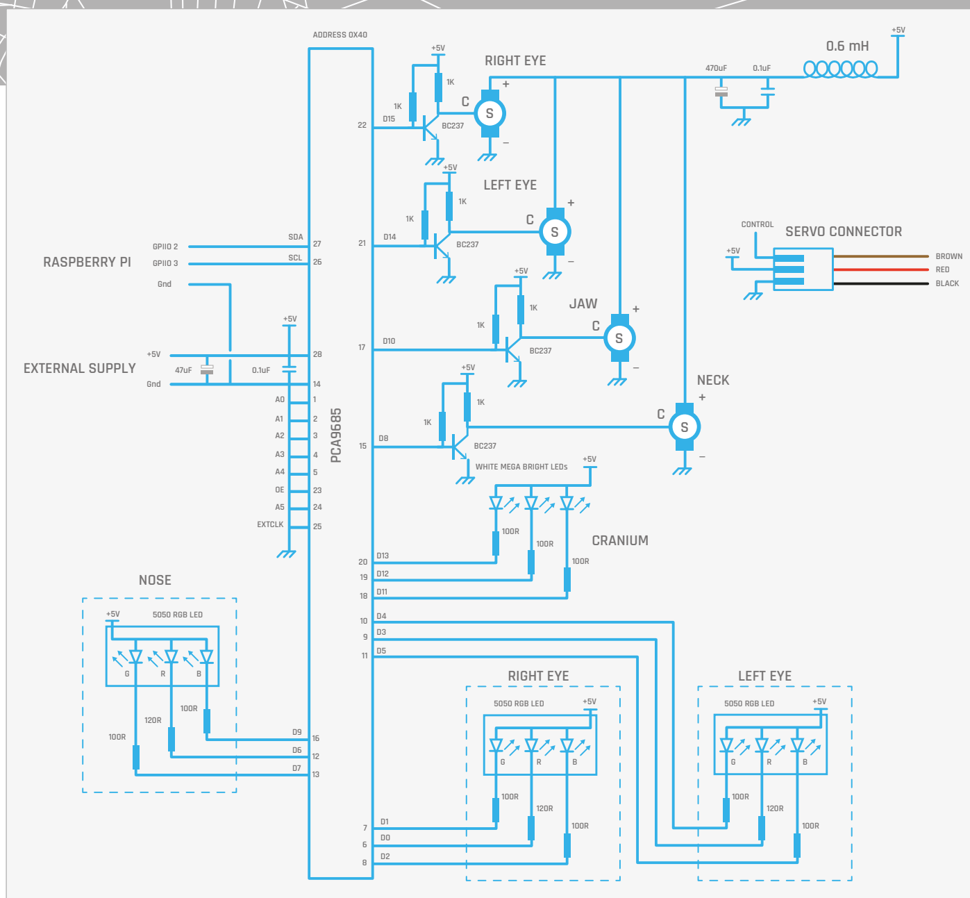
Fig. 2 The schematic of Mulder
