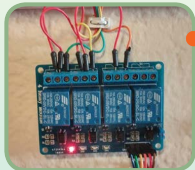
The SainSmart relay is wired between the Raspberry Pi and the HVAC control unit
