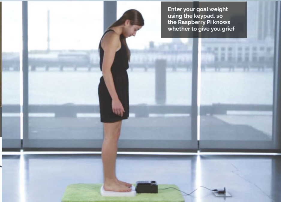
A Raspberry Pi is hooked up to the scale and speakers to provide audio feedback
