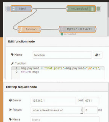
Your first flow: the code you need to write into your function node, and configuration details for the TCP request node
