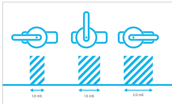
Above Controlling a servo motor
