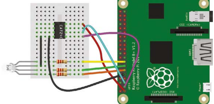
Fig 2 To test your HAT, make sure you reconnect the EEPROM so that it is wired to ID_SC and ID_SD. You also need to add two pull-up resistors
