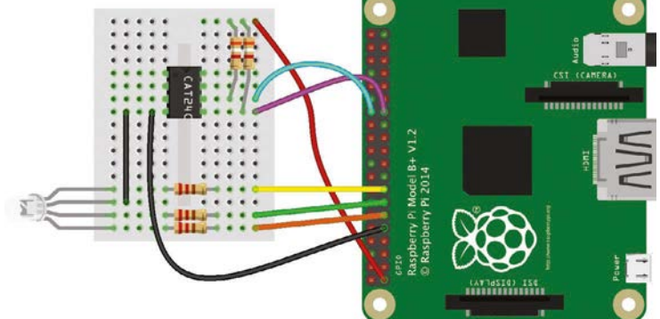
Fig 2 To test your HAT, make sure you reconnect the EEPROM so that it is wired to ID_SC and ID_SD. You also need to add two pull-up resistors
