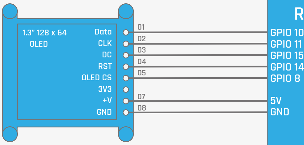
Fig 1 Connecting the OLED display to the Raspberry Pi
