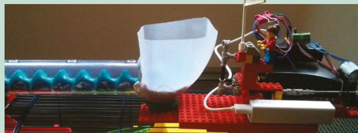
Below The overall layout, showing the Archimedes screw and hopper with motor and gears
