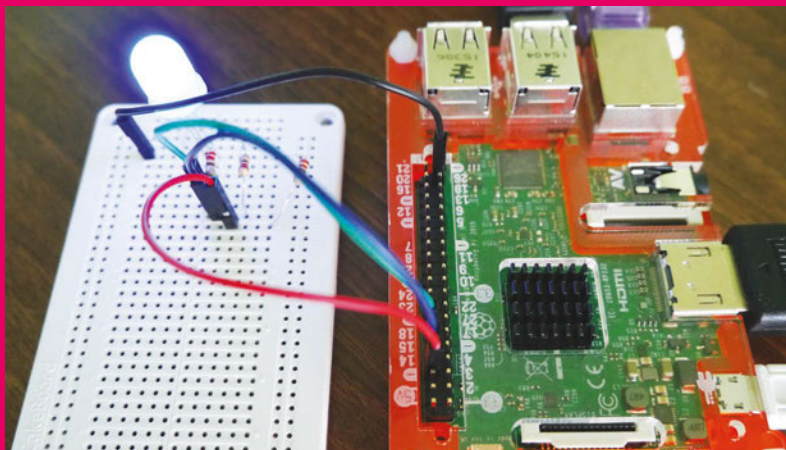
The CPU monitor in action. Chunky 10mm LEDs make a big, bright indicator
