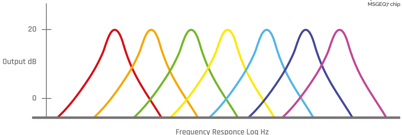
Fig 1 The frequency response of the MSGEQ7 chip
