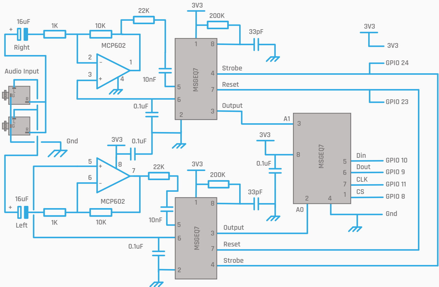
Fig 2 The schematic of the Spectrum board
