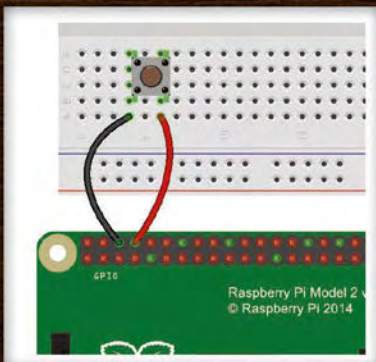
Fig 1 It's very simple to wire up a button to the Raspberry Pi
