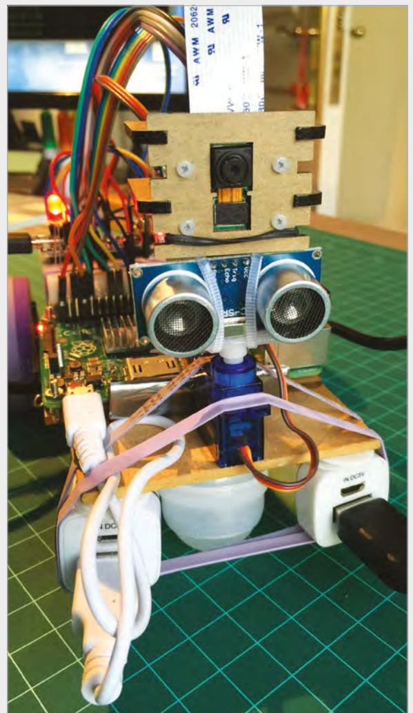
Above The finished robot looks ready for lift-off (or at least ready to explore the back garden)
