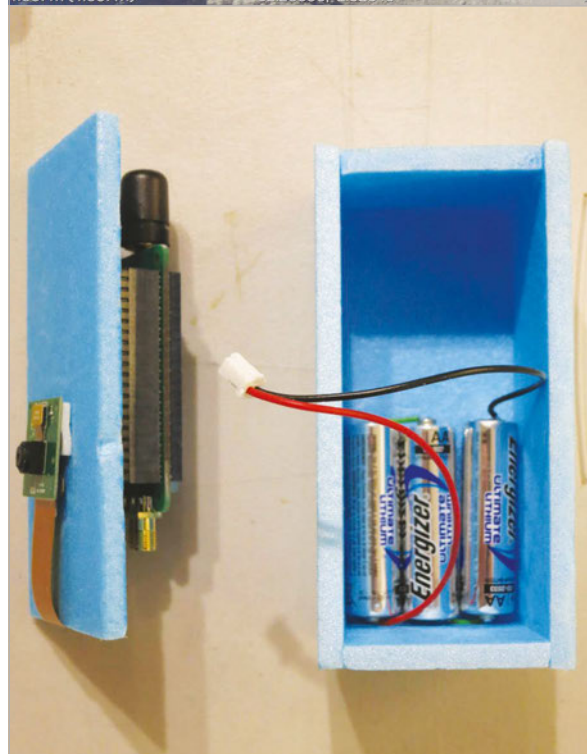
A basic case with the bare essentials needed to make things work, which is important when you're trying to save weight
