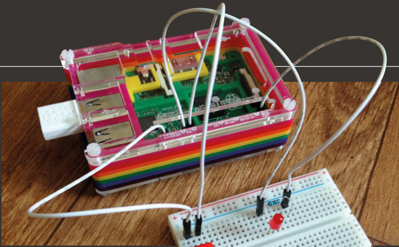
The simple breadboard circuit is connected to the GPIO pins on the Raspberry Pi
